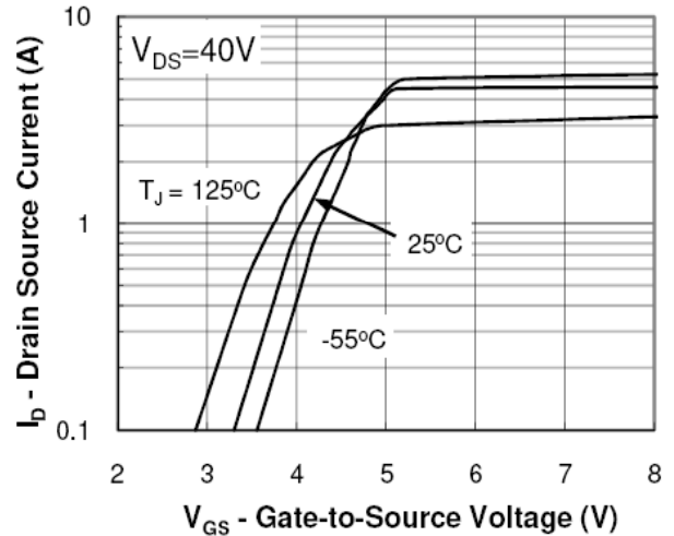
Transfer Characteristic
