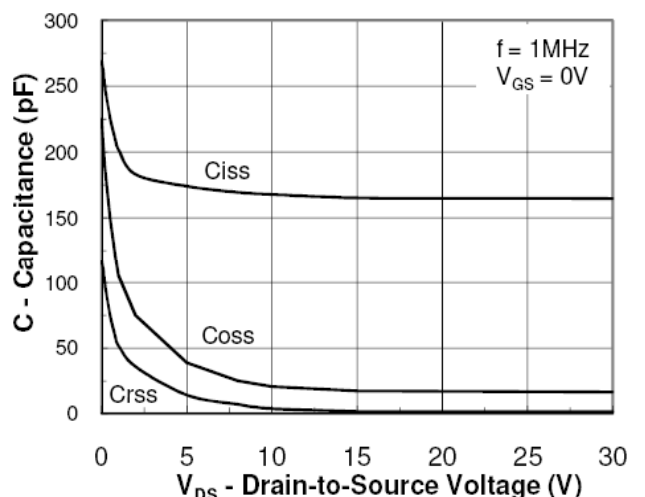
Capacitance
