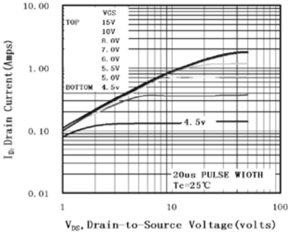
Output Characteristic
