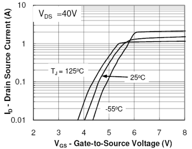
Transfer Characteristic
